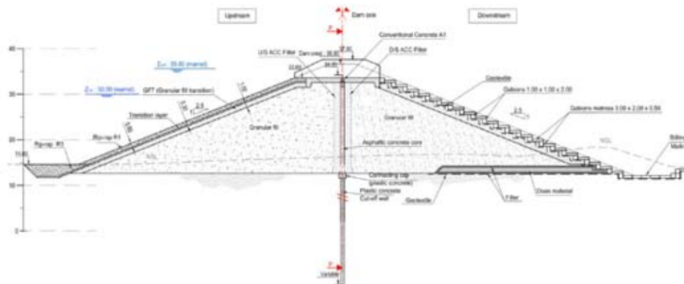
Figure 6 : Cross section through the embankment dam with gabions on the downstream slope of the dam.
