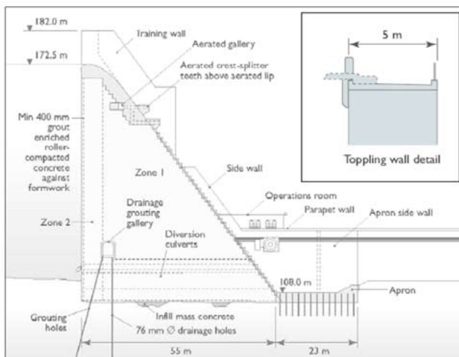
Figure 4 . Cross section through the Wadi Dayqah RCC Dam with the toppling crest elements (taken from Hieatt et al., 2010).
